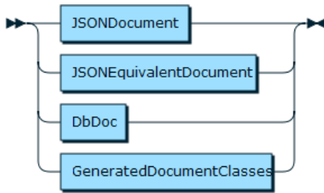
Figure 11.39 Document
