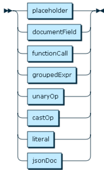
Figure 12.19 atomicExpr
