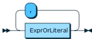
Figure 11.30 ExprOrLiterals
