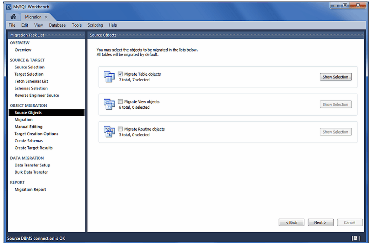
Figure 10.55 MySQL Workbench migration: Source Objects
