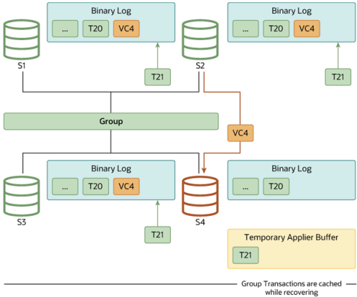
Figure 20.11 Queued Transactions
