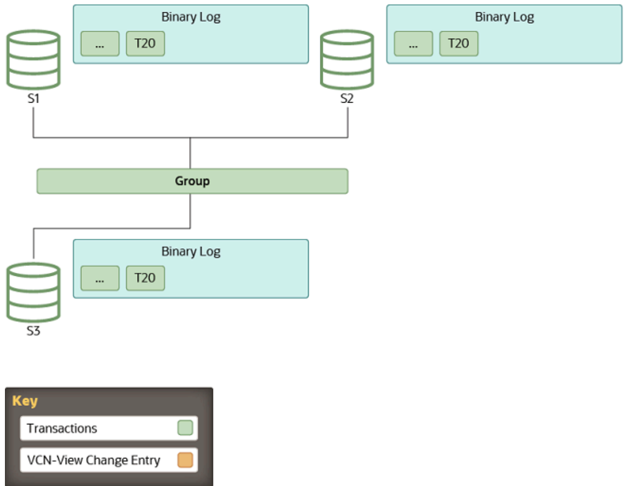
Figure 20.8 Stable Group
