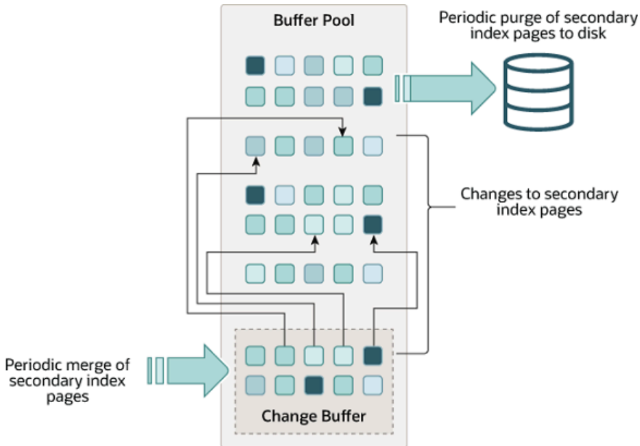
Figure 17.3 Change Buffer
