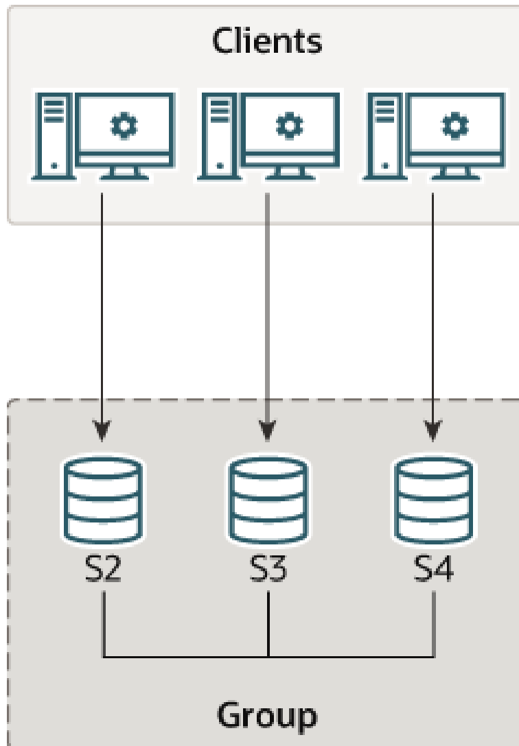
Figure 20.7 Group Architecture
