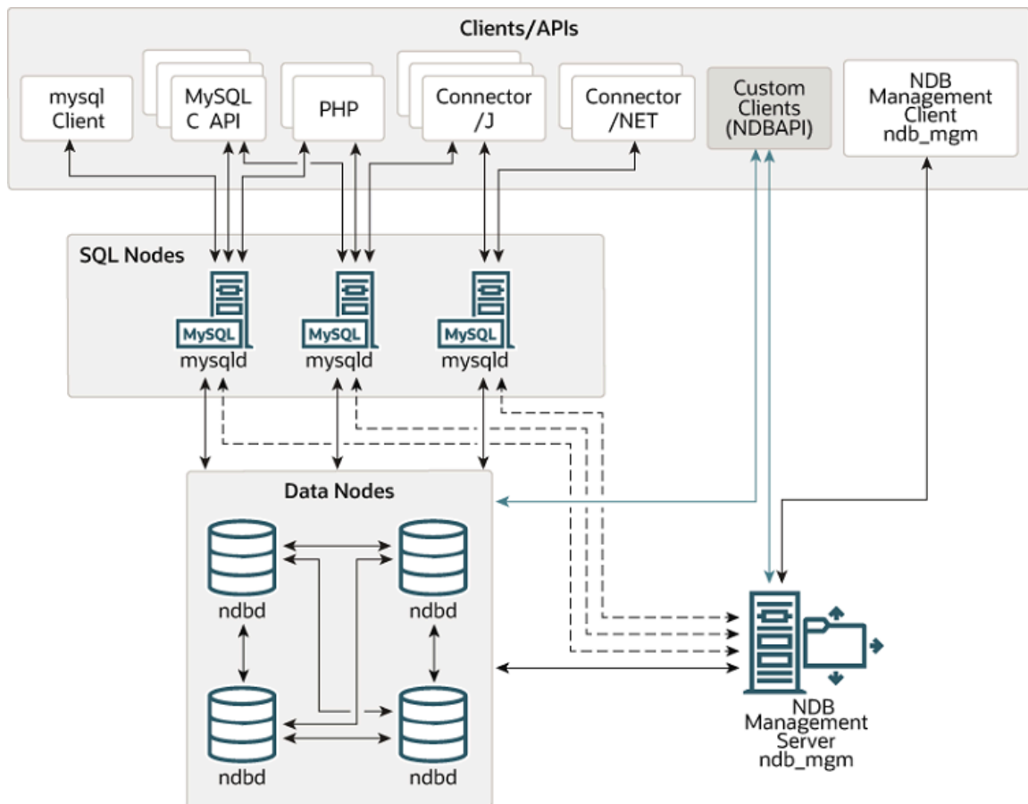
Figure 23.1 NDB Cluster Components
