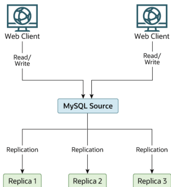
Figure 17.4 Redundancy Using Replication, Initial Structure
