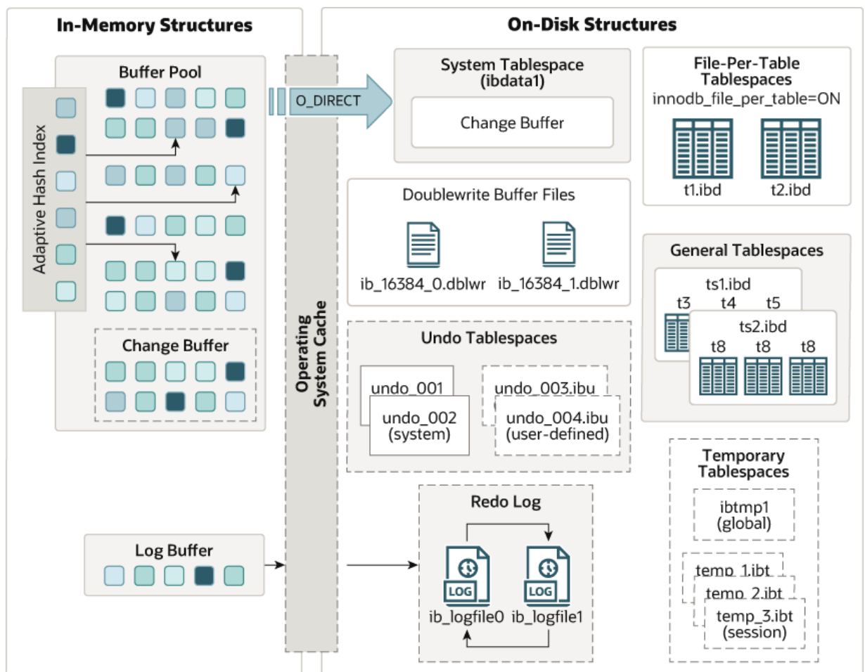
Figure 15.1 InnoDB Architecture
