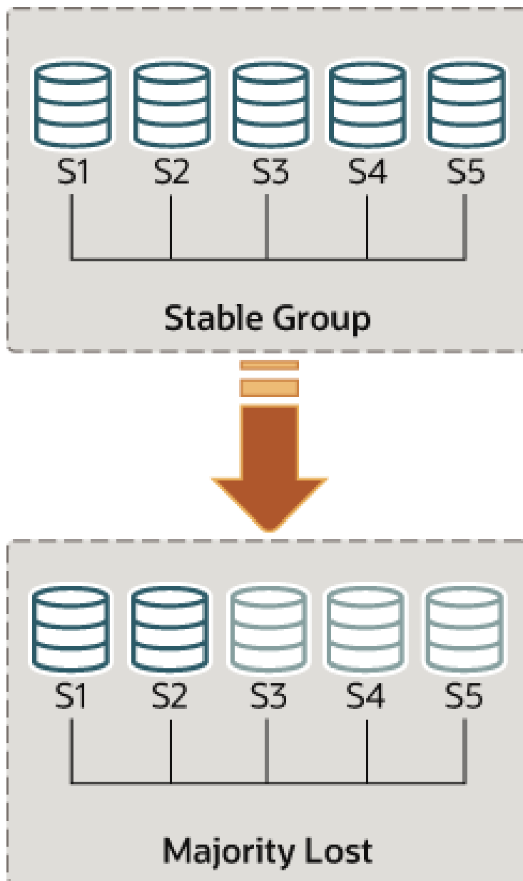
Figure 18.14 Losing Quorum
