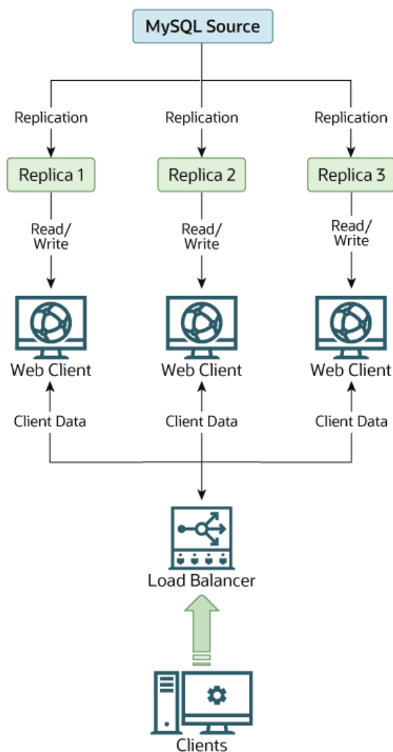
Figure 17.1 Using Replication to Improve Performance During Scale-Out
