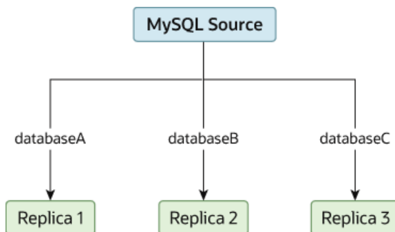
Figure 17.2 Replicating Databases to Separate Replicas
