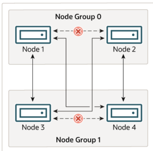
Figure 23.3 Nodes Required for a 2x2 NDB Cluster
