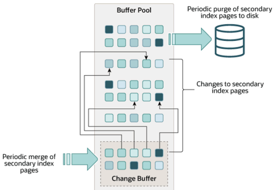
Figure 15.3 Change Buffer
