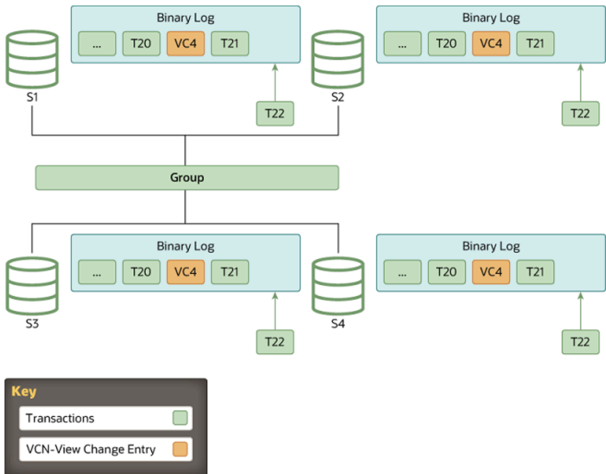
Figure 18.12 Instance Online
