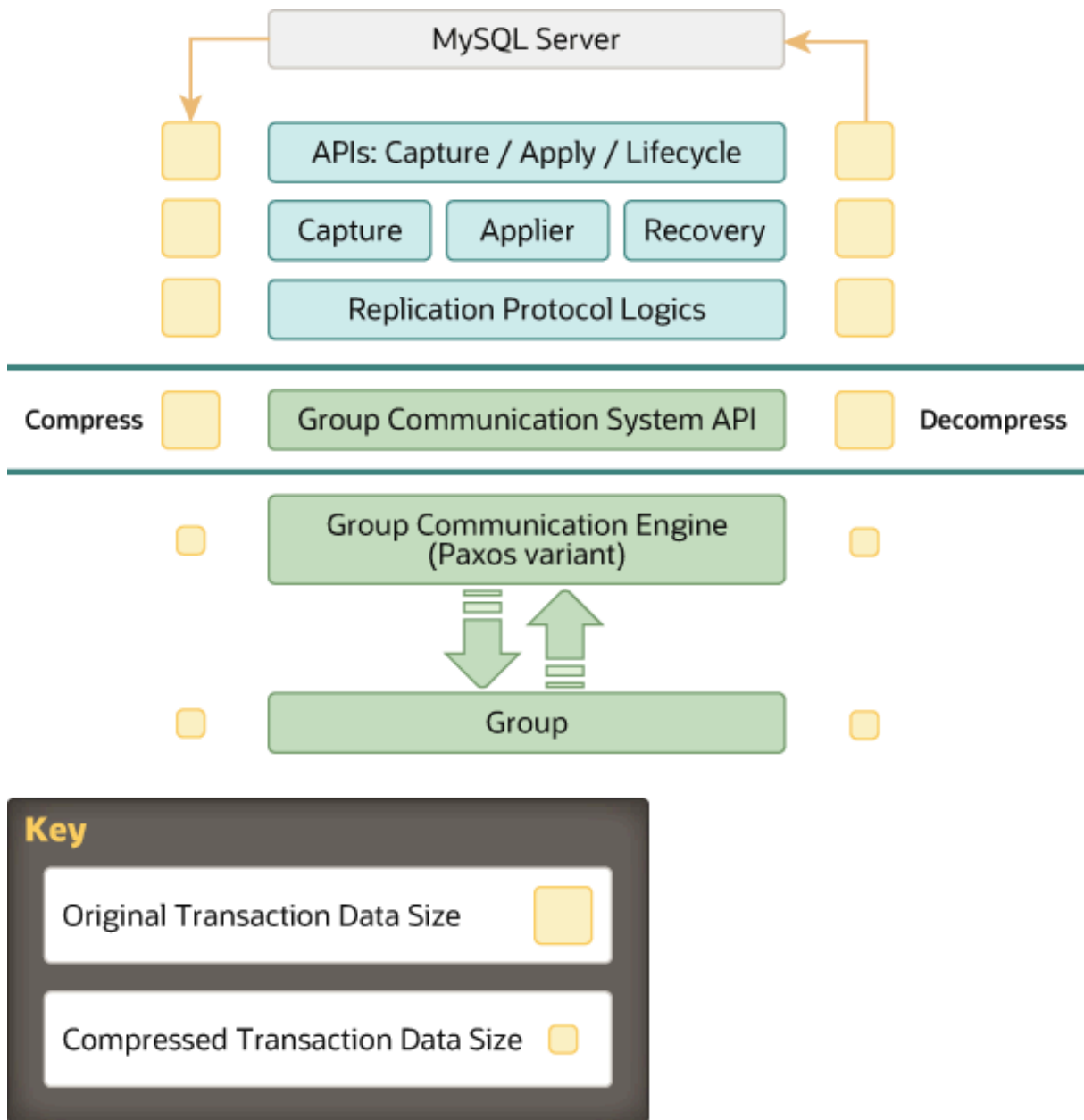
Figure 18.13 Compression Support
