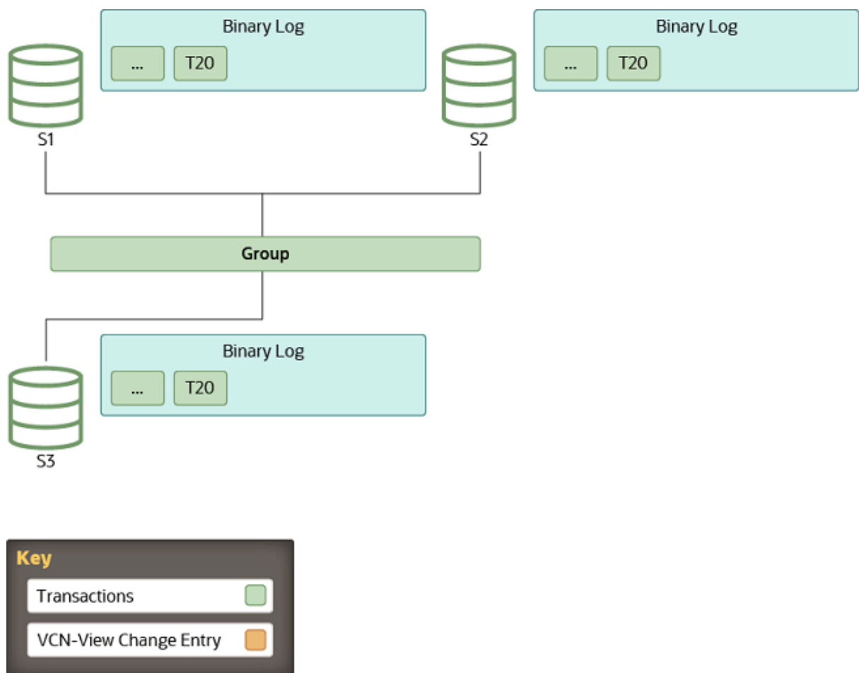
Figure 18.8 Stable Group
