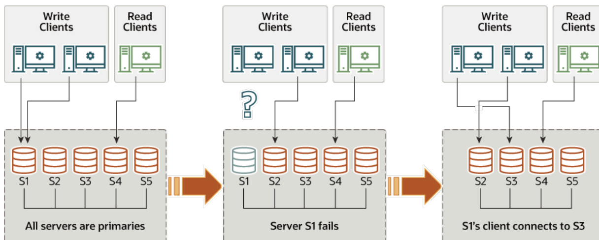
Figure 18.5 Client Failover
