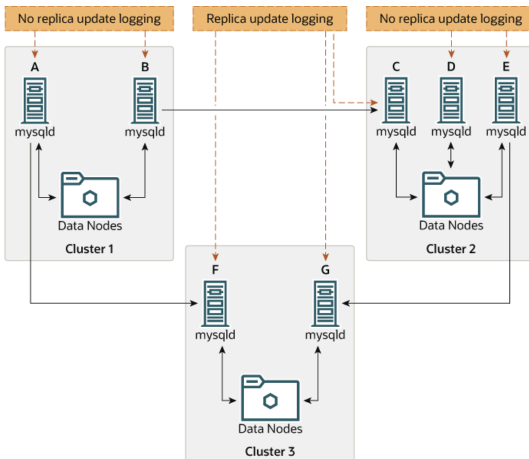
Figure 23.17 NDB Cluster Multi-Source Replication, With MySQL Servers
