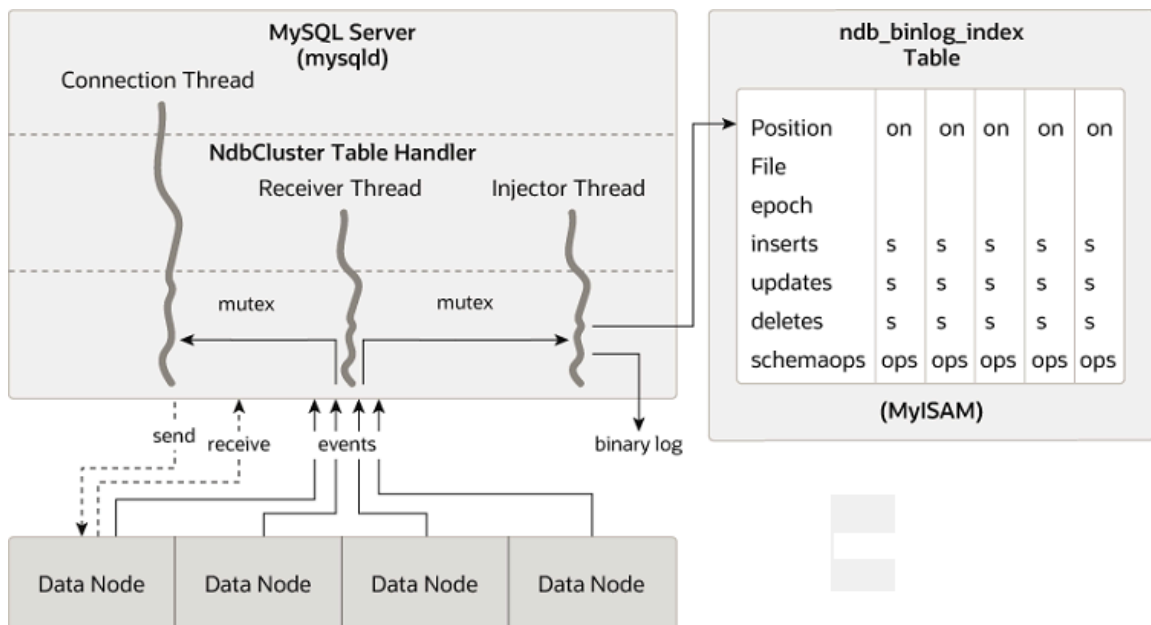
Figure 23.13 The Replication Source Cluster
