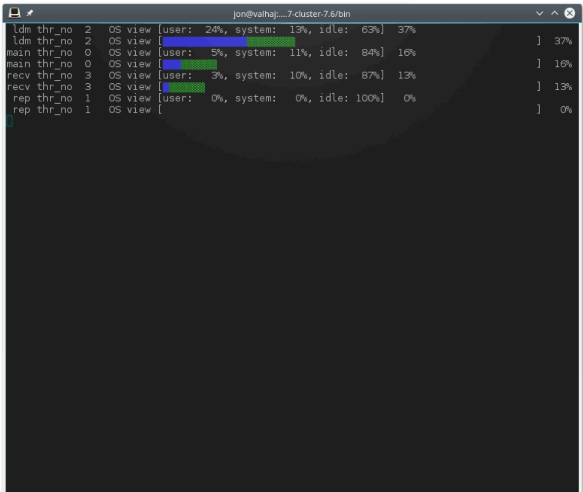
Figure 23.5 ndb_top Running in Terminal
