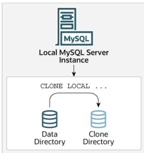
Figure 5.1 Local Cloning Operation
