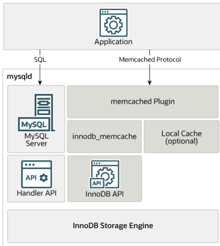
Figure 15.4 MySQL Server with Integrated memcached Server
