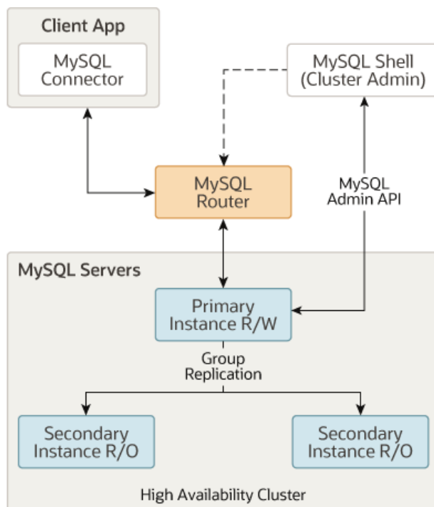
Figure 21.1 InnoDB Cluster overview
