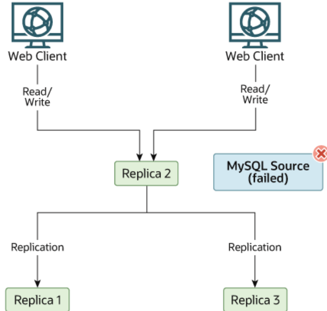
Figure 17.5 Redundancy Using Replication, After Source Failure
