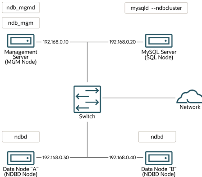
Figure 23.4 NDB Cluster Multi-Computer Setup
