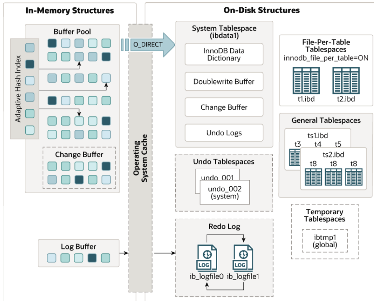
Figure 14.1 InnoDB Architecture
