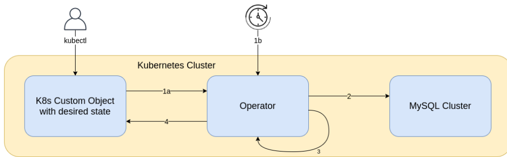
Figure 1.1 NDB Operator reconciliation loop
