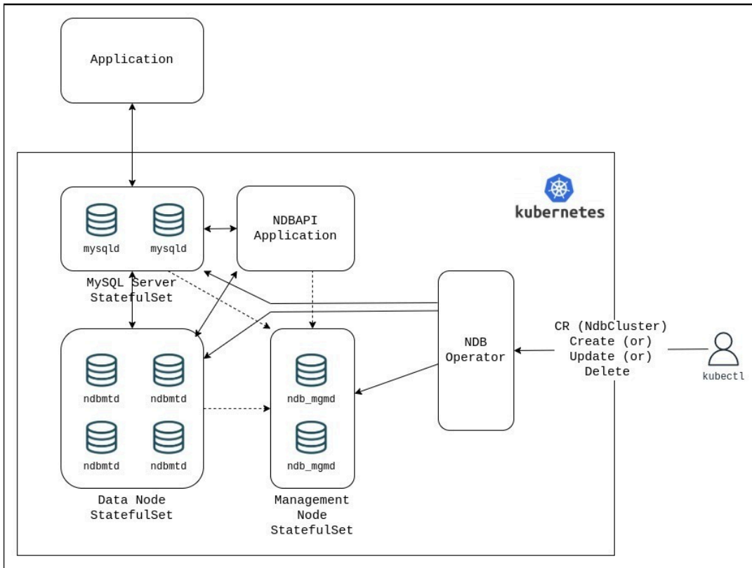
Figure 1.2 NDB Operator architecture
