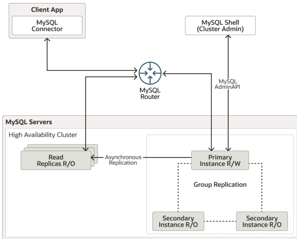
Figure 8.3 InnoDB Cluster Read Replicas overview
