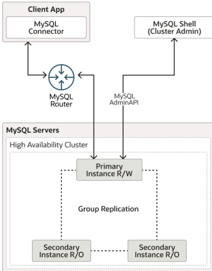
Figure 8.1 InnoDB Cluster overview
