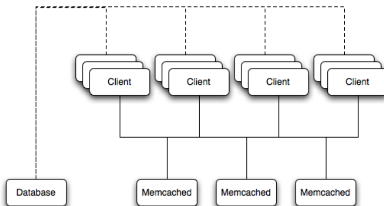
Figure 1.1 memcached Architecture Overview
