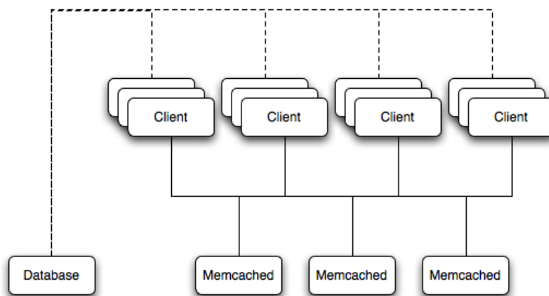
Figure 1.1 memcached Architecture Overview
