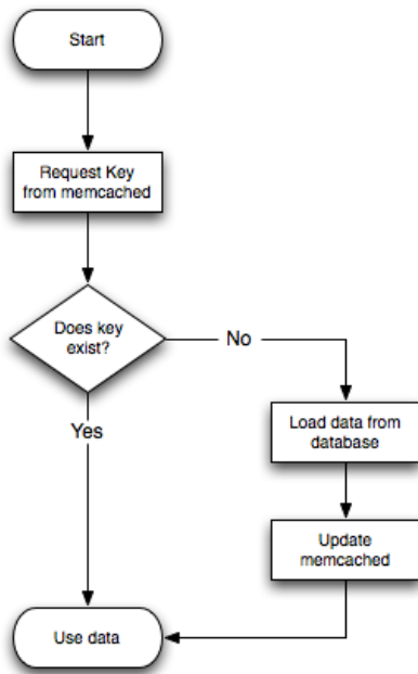
Figure 4.1 Typical memcached Application Flowchart
