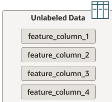
Figure 4.3 Unlabeled Data
