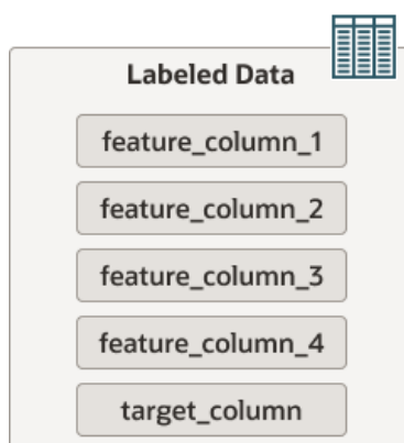
Figure 4.2 Labeled Data
