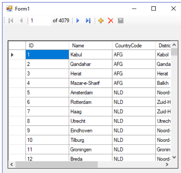
Figure 6.17 The Populated Grid Control
